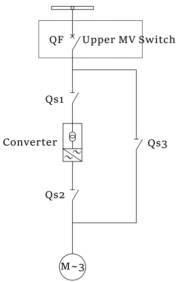
Scheme of one for one + manual bypass 10KV MV bus
