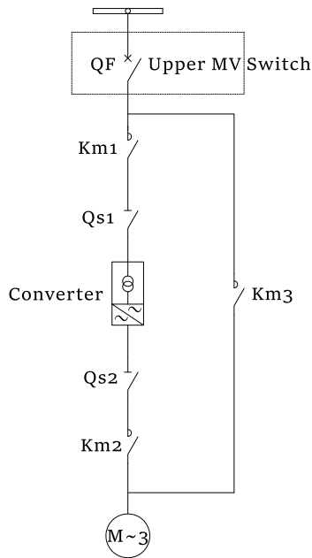
Scheme 2 of one for two
